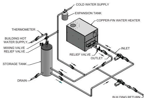
Figure 2-2_Vertical Tank Piping Diagram, Non-Condensing
