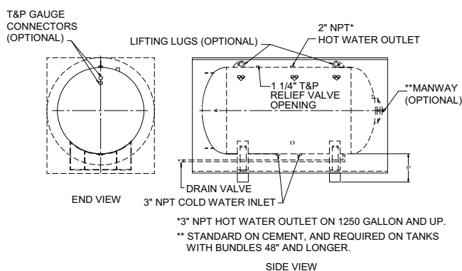
Figure 5-2_Horizontal Tank
