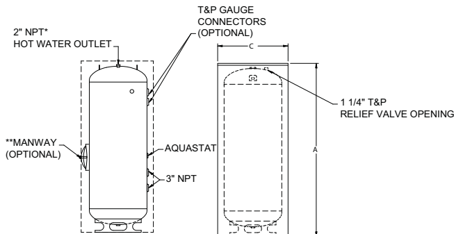
Figure 5-1_Vertical Tank
