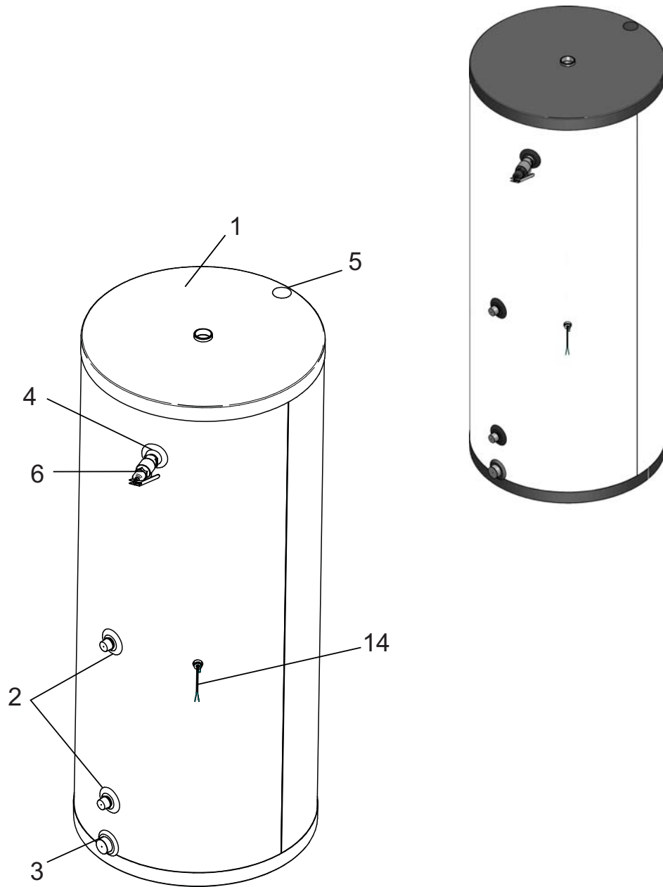
STAINLESS STEEL INDIRECT TANK (SIT_SIT DW)
