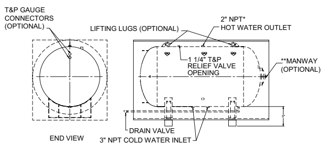
Figure 5-2_Horizontal Tank
