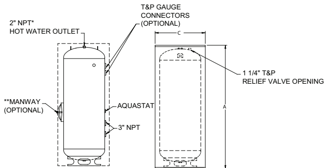
Figure 5-1_Vertical Tank
